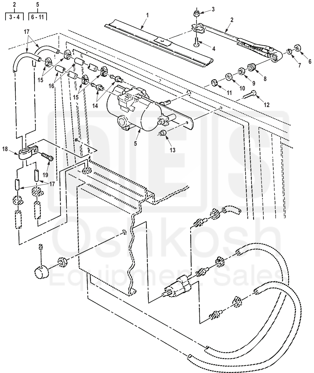
Figure 552. Windshield Wiper Arm, Blade, and Motor Assembly (New Style).
